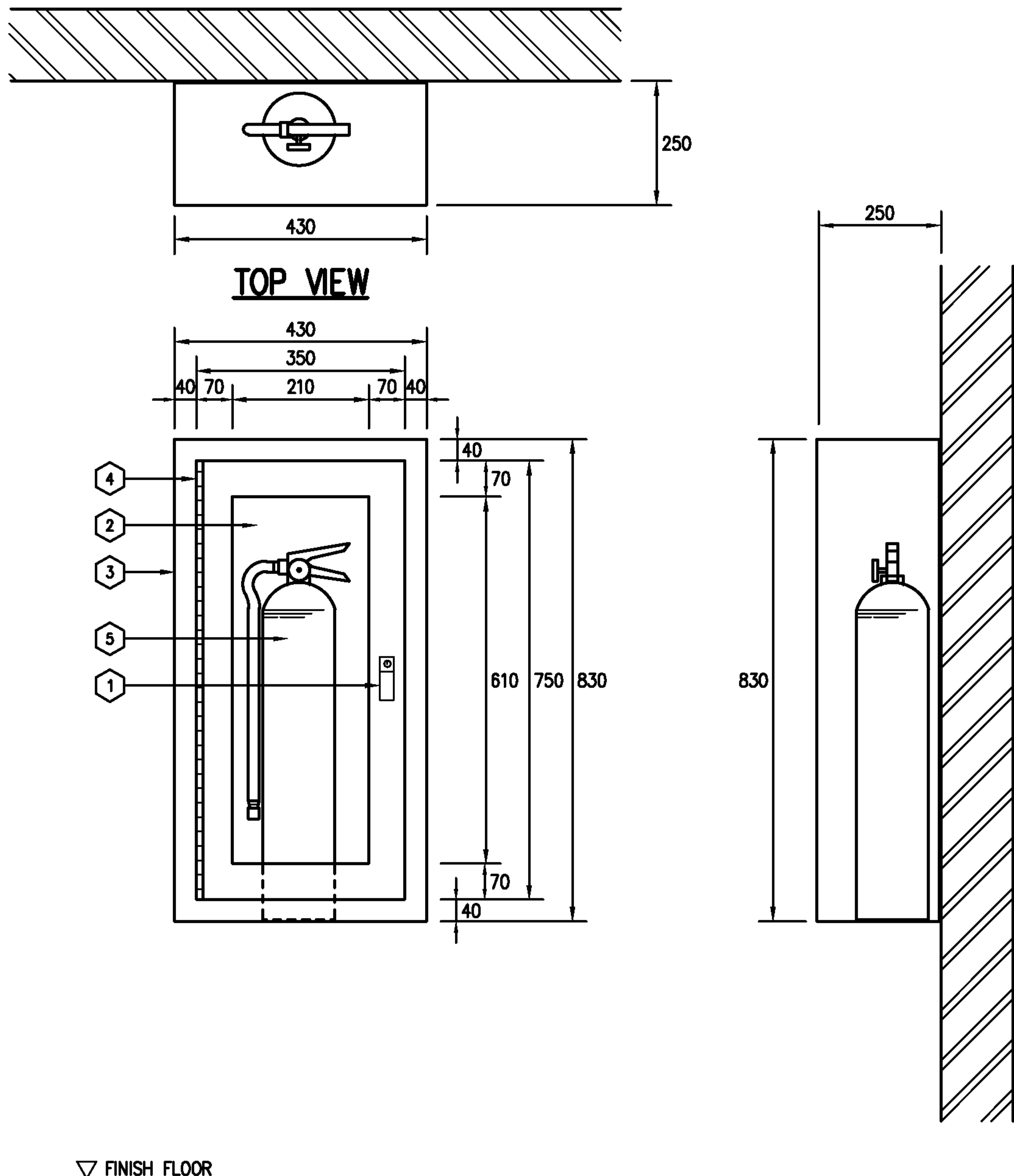
FRONT VIEW
