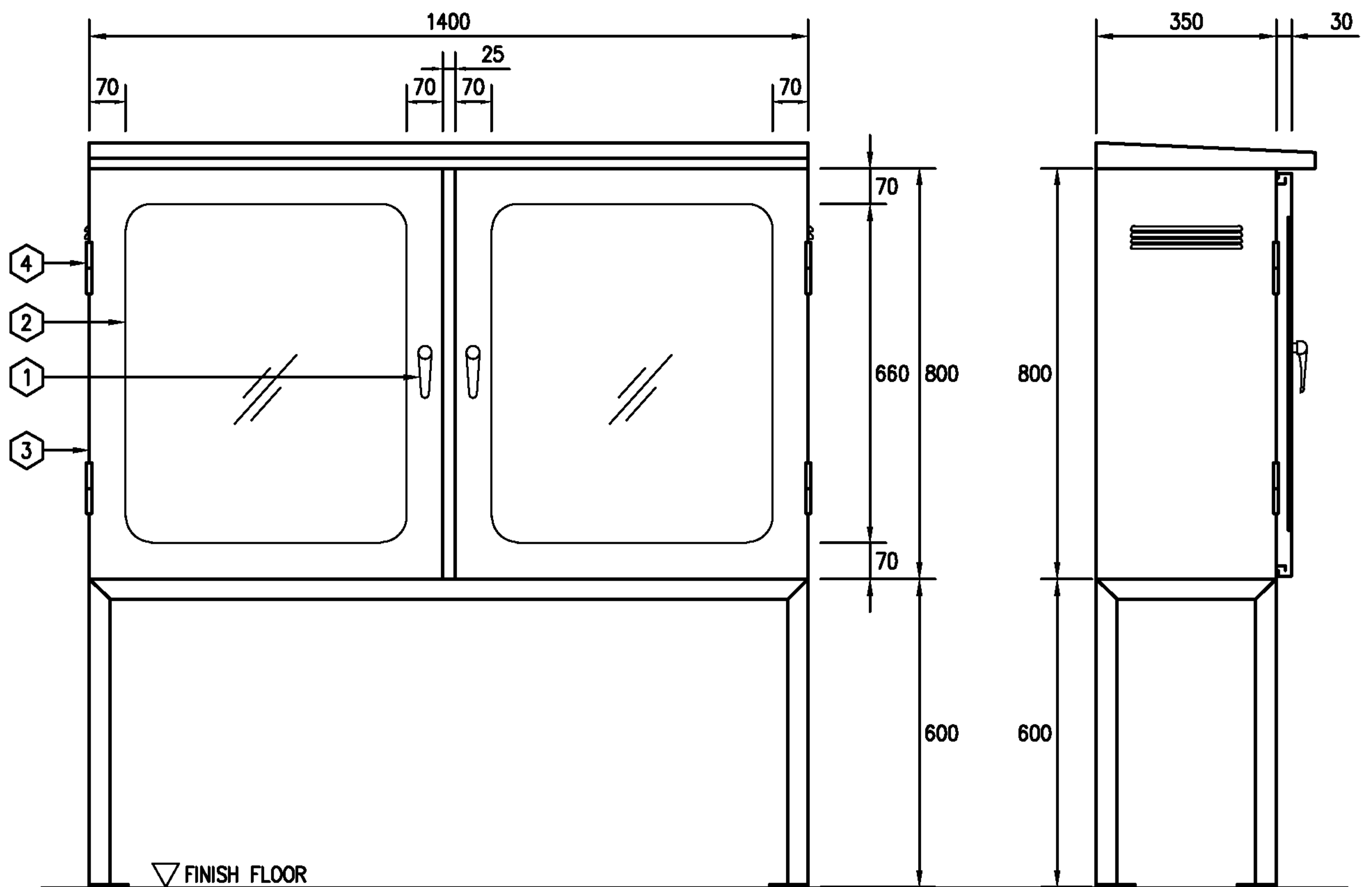
FRONT VIEW
