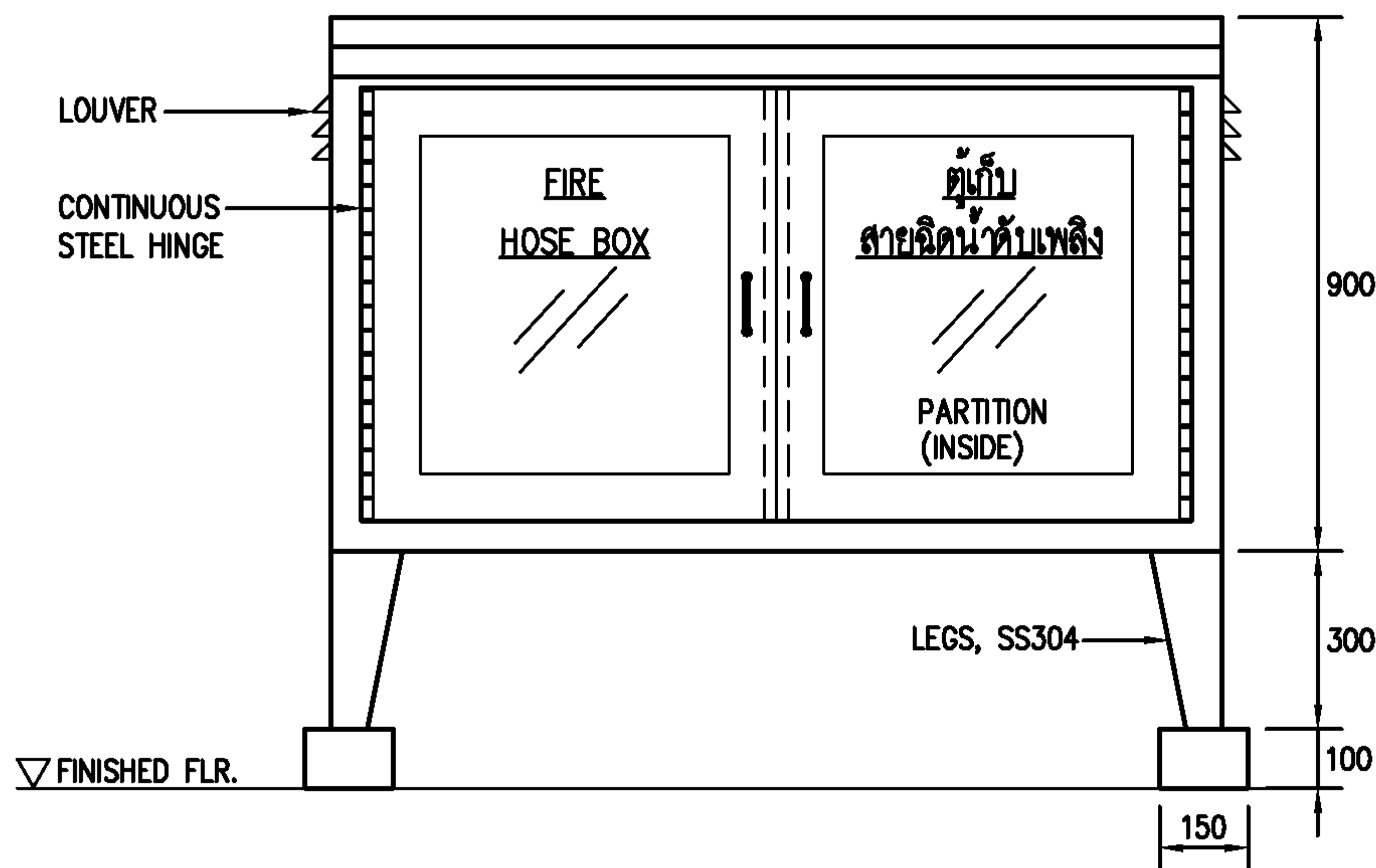
FRONT VIEW
