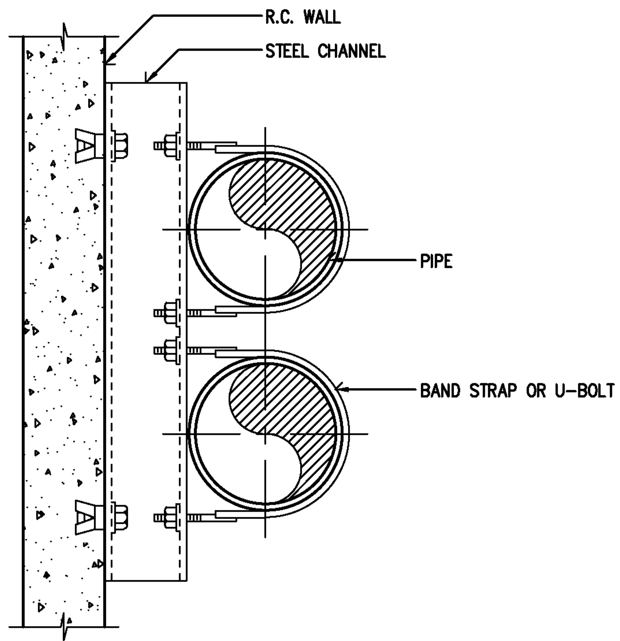
PLAN
