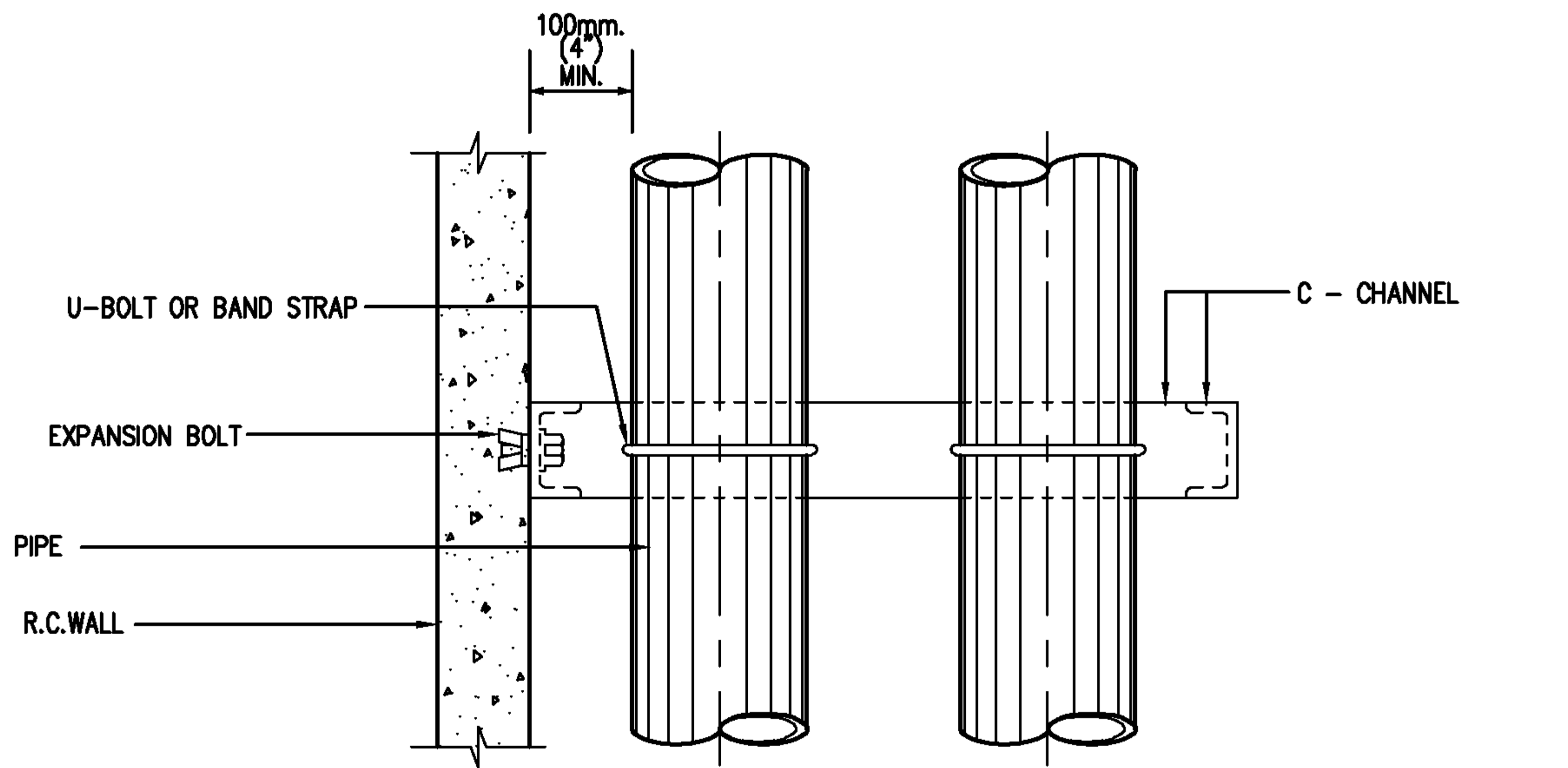
PLAN
